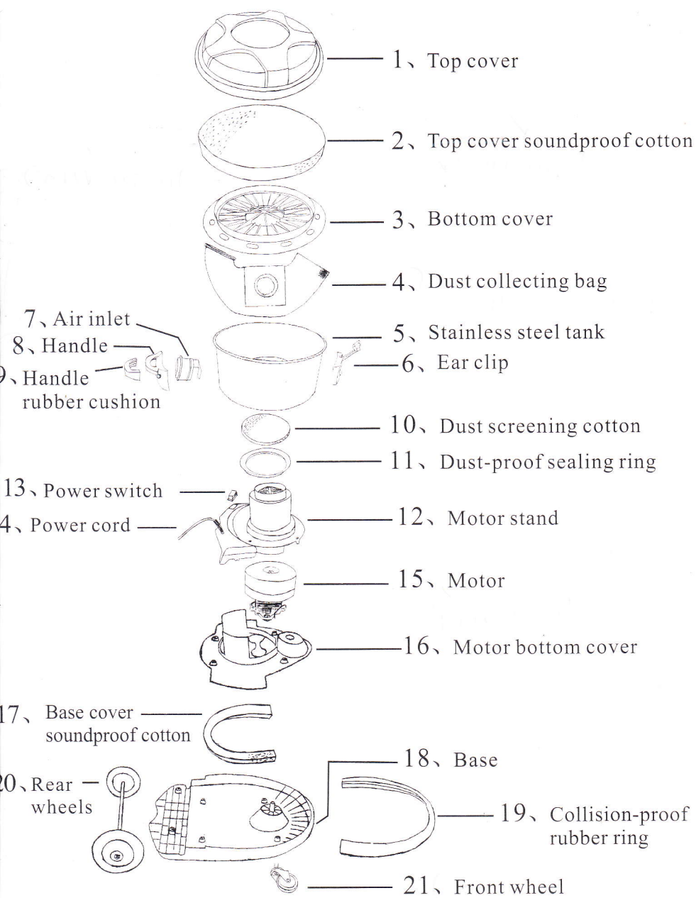
10-liter Low-noise Industrial and Commercial Vacuum Cleaner Breakdown Figure
