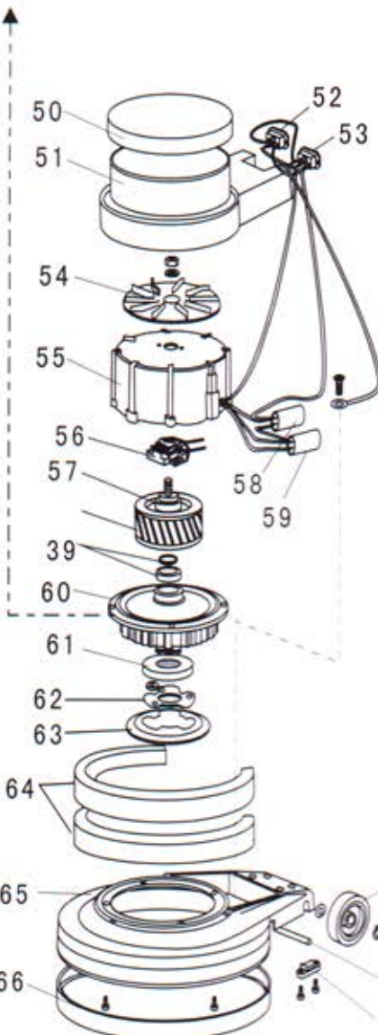
BF523/523A/523B EXPLODED VIEW
