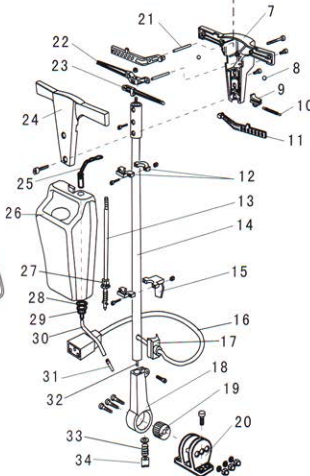
BF523 EXPLODED VIEW
