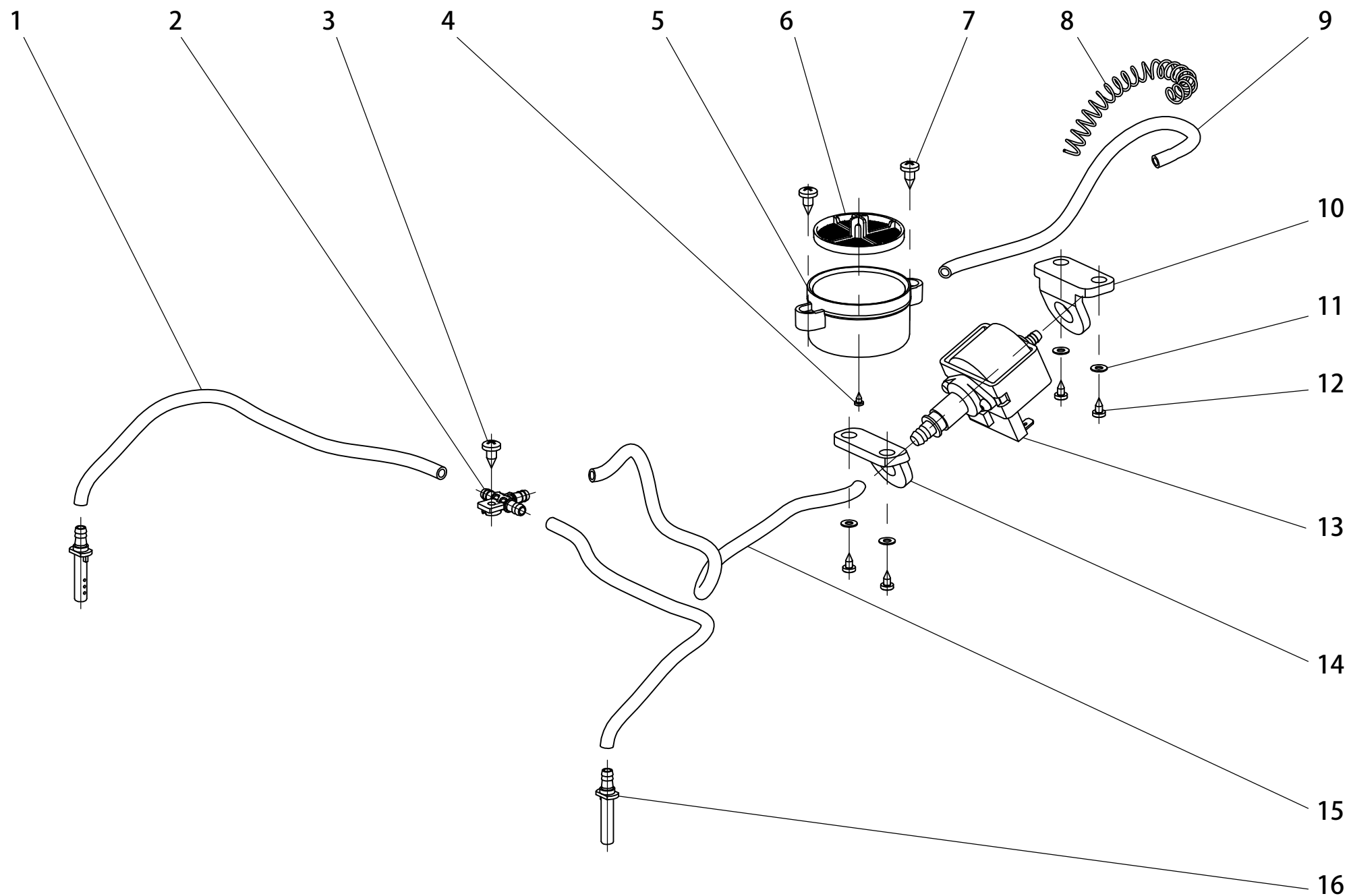
11.water releasing part Assembly
