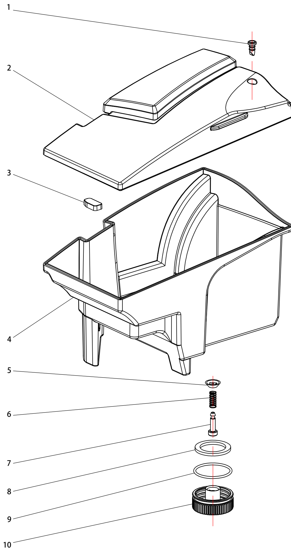
4.Fresh Water tank Assembly
