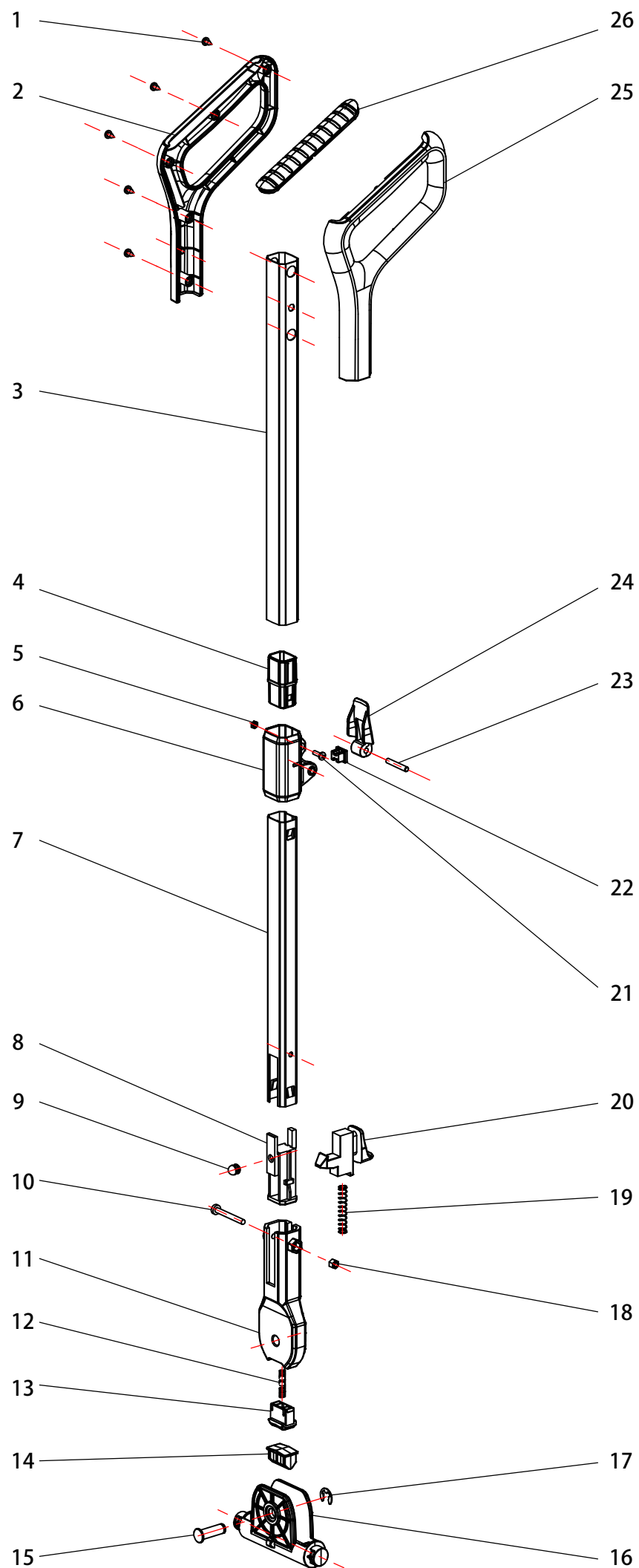
10.Handle Assembly
