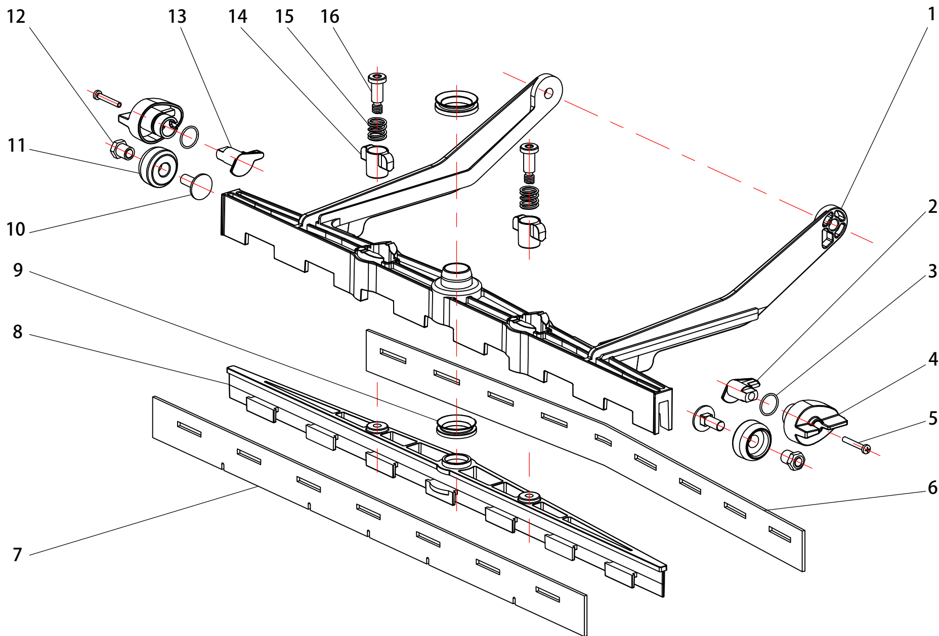
9.Squeeze Assembly
