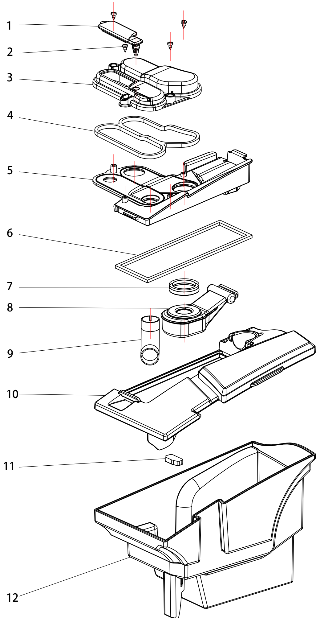
5.Dirty water tank Assembly
