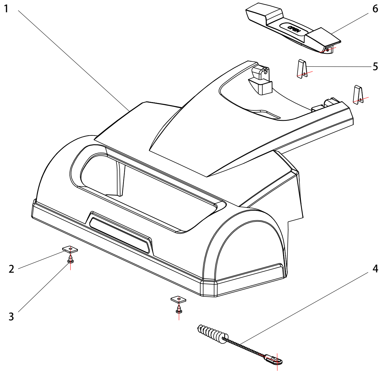
8.Front Cover Assembly
