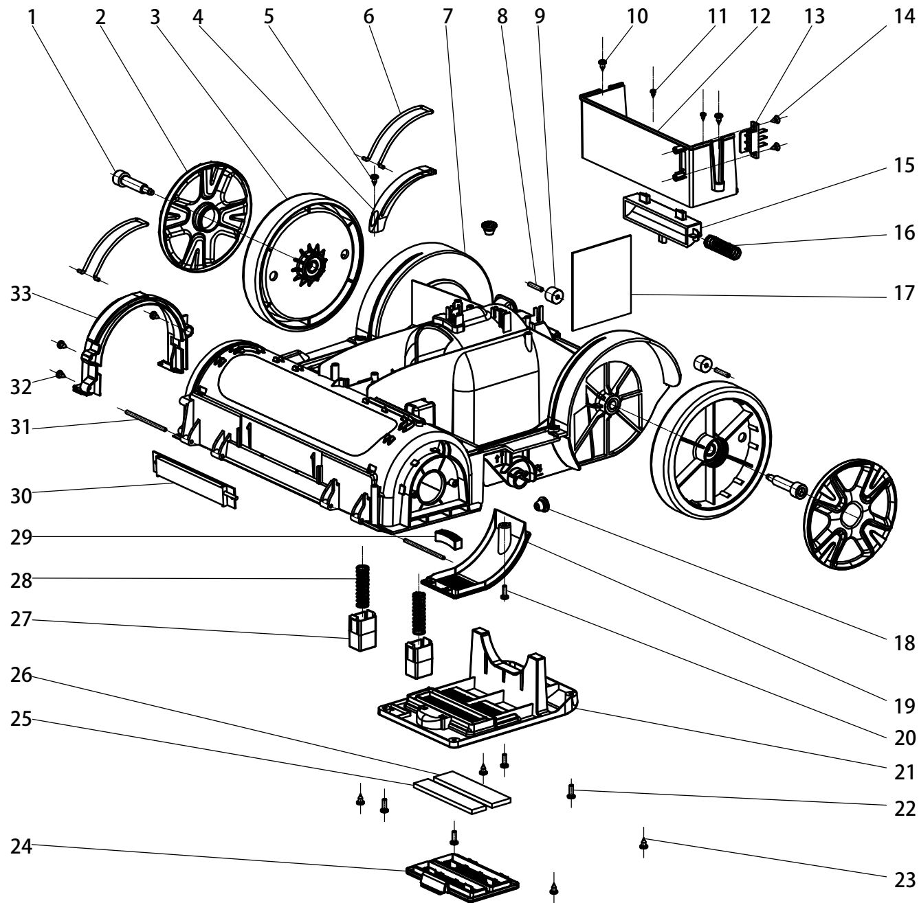
1.Chasis Assembly
